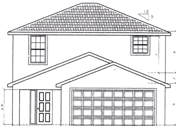
FRONT ELEVATION 1/4" = 1'-0"
