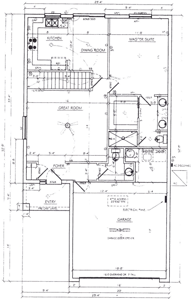
FLOOR PLAN 1/4" = 1'-0"
